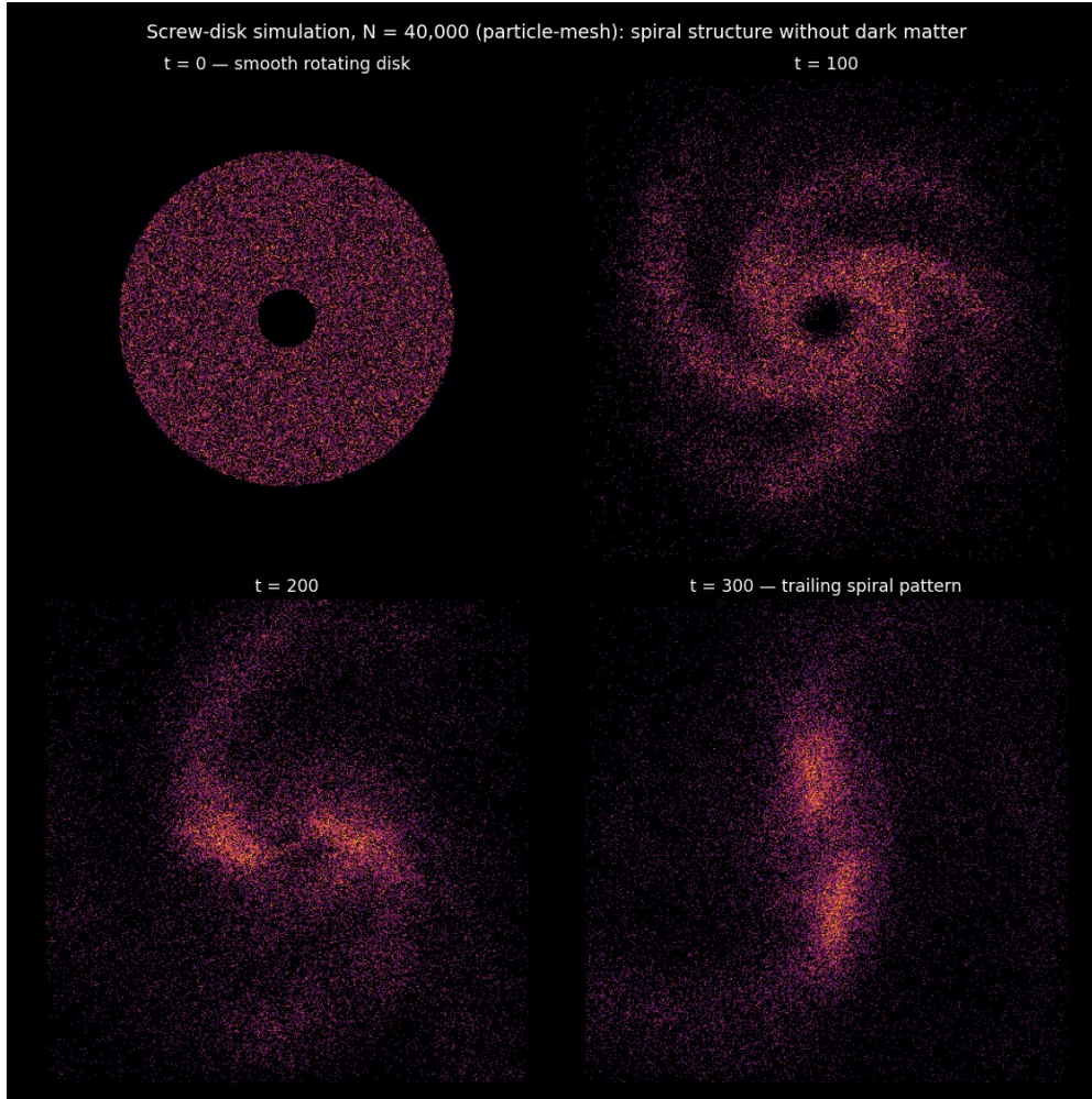
Figure 2. Stage B evolution ( N = 40,000 , particle-mesh method): the smooth rotating disk (upper left) develops a multi-armed spiral phase ( t = 100 ) through swing amplification of its own gravity, then coarsens into a dominant two-armed mode — the expected fate of a collisionless run; in real galaxies the gas cycle regenerates the fine-armed phase continuously. All parameters are stated in the text; the simulation program accompanies this paper.
