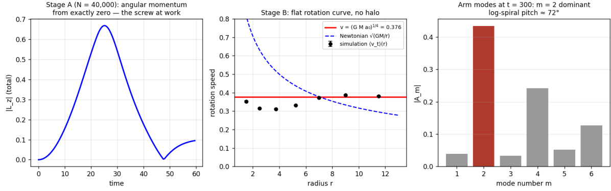
Figure 1. Left: total angular momentum in Stage A, starting from exactly zero — the screw converts gravitational infall into rotation with fixed handedness. Middle: the Stage B rotation curve (points) against the parameter-free screw prediction v = (G M a_0)^{1/4} (solid) and the Newtonian expectation for the same visible mass (dashed). Right: Fourier mode analysis of the final pattern; the two-armed mode dominates.
